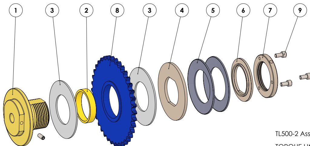
TORQUE LIMITER
