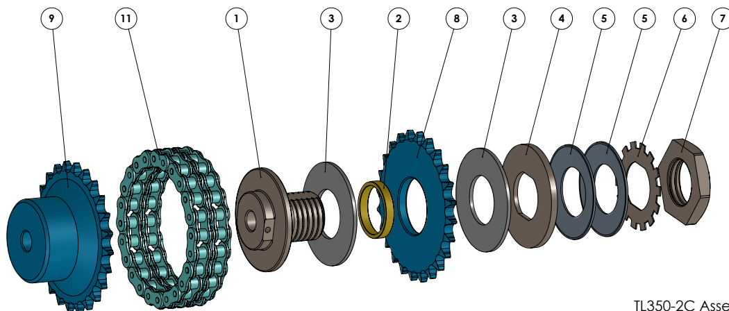
TL350-2C Assembly
